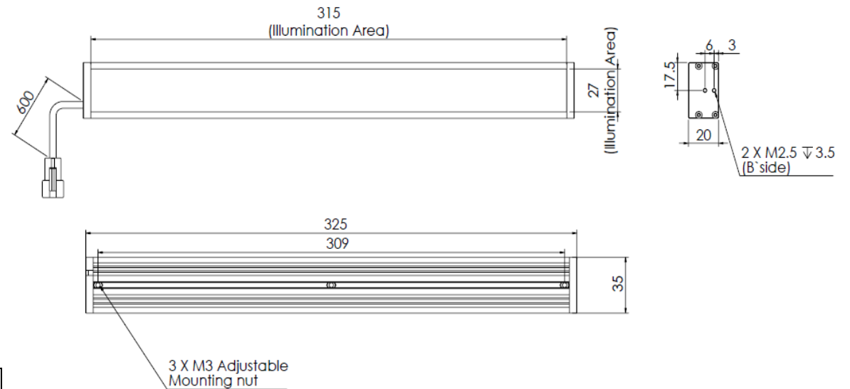
Lighting Dimension
